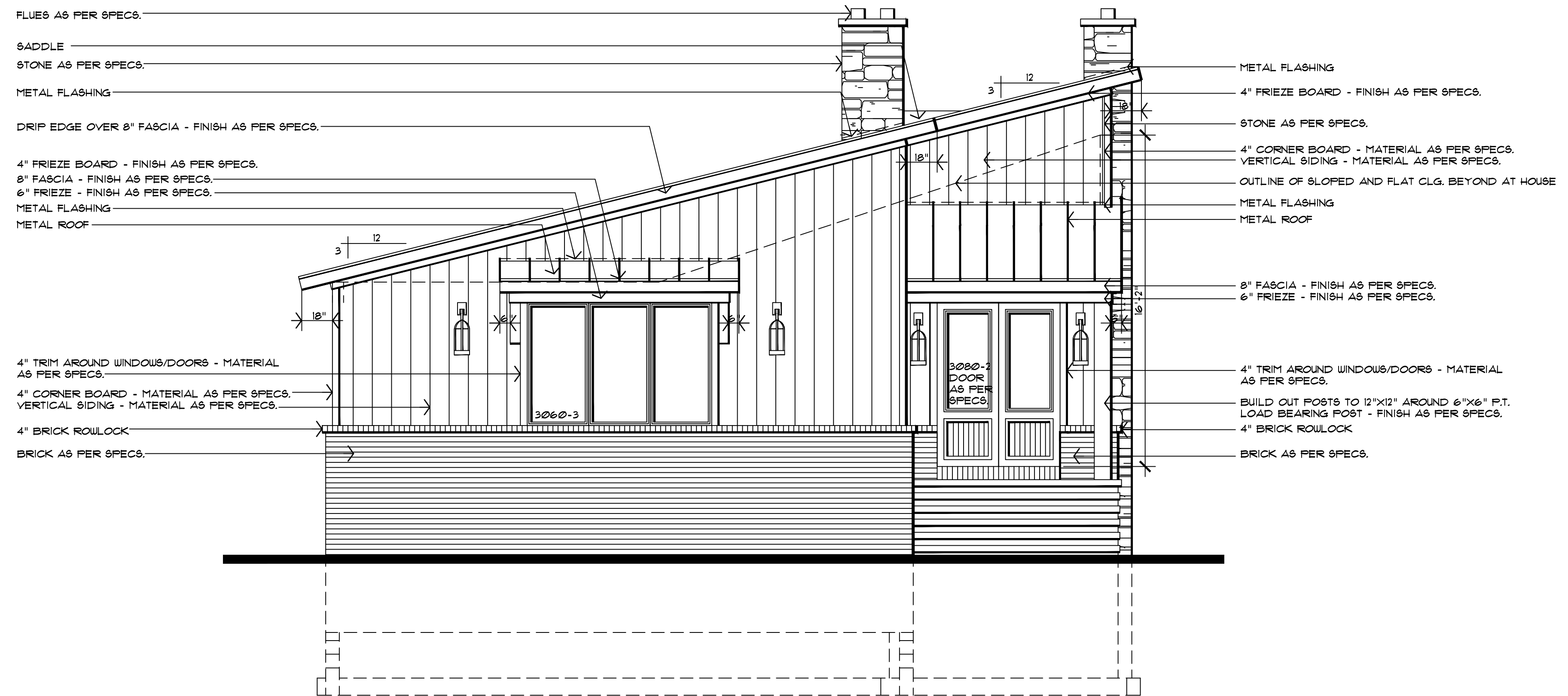
ROADSIDE (REAR) ELEVATION
